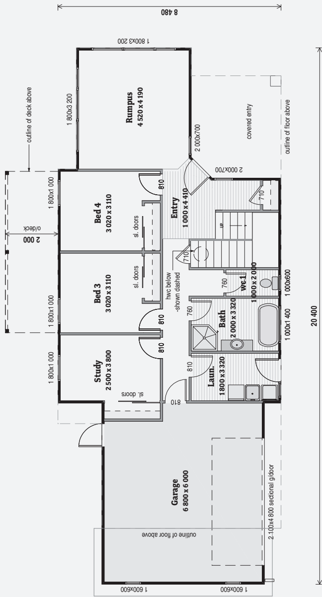
Ground Floor Area 137.0m 2 o/frame
